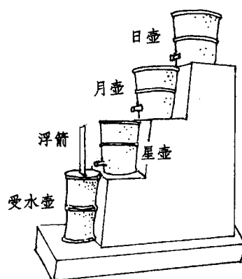
漏壶
